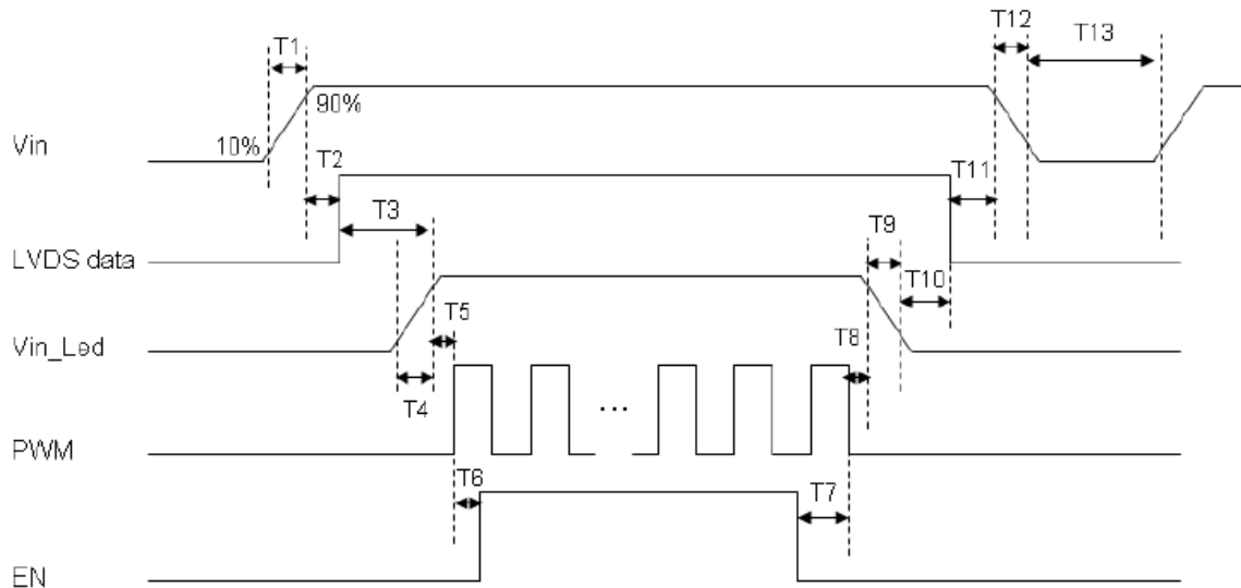
Power Sequence
